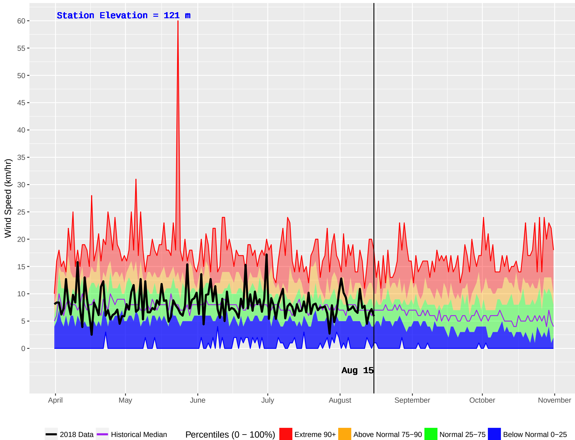
BOWSER (56) : Historical (1985–2016) and Current (2018) Daily Wind Speed
