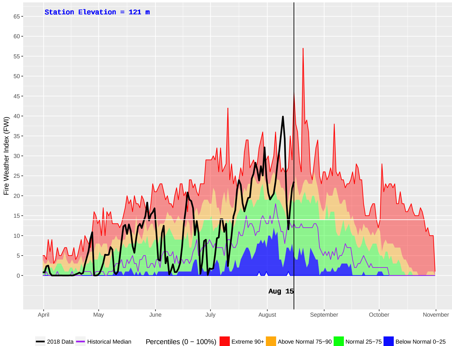
BOWSER (56) : Historical (1985–2016) and Current (2018) Daily Fire Weather Index (FWI)
