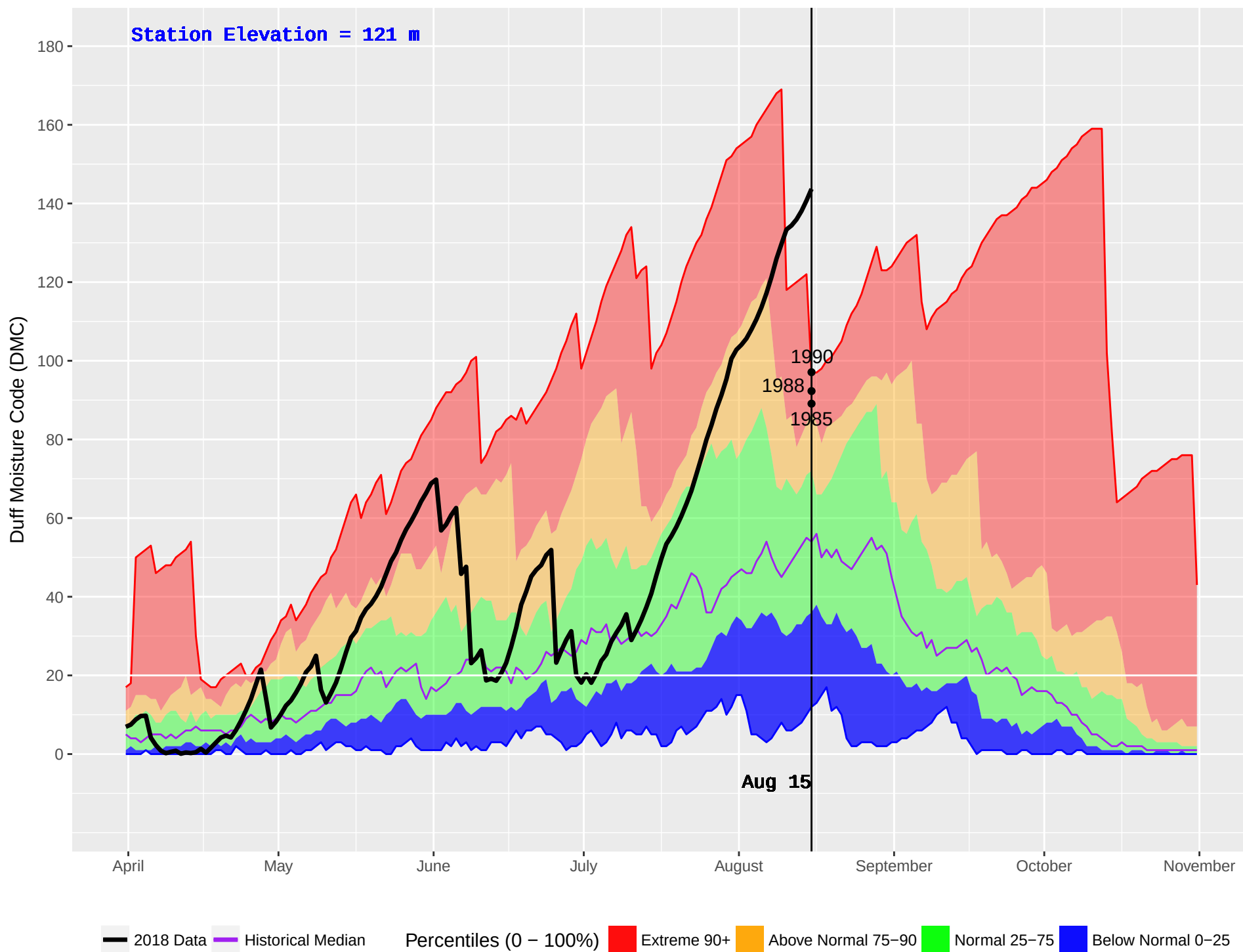
BOWSER (56) : Historical (1985–2016) and Current (2018) Daily Duff Moisture Code (DMC)
