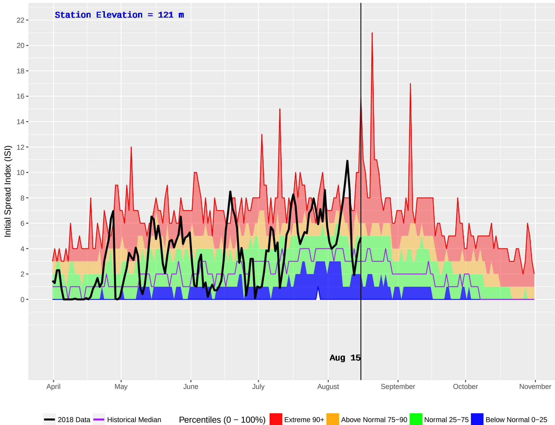
BOWSER (56) : Historical (1985–2016) and Current (2018) Daily Initial Spread Index (ISI)
