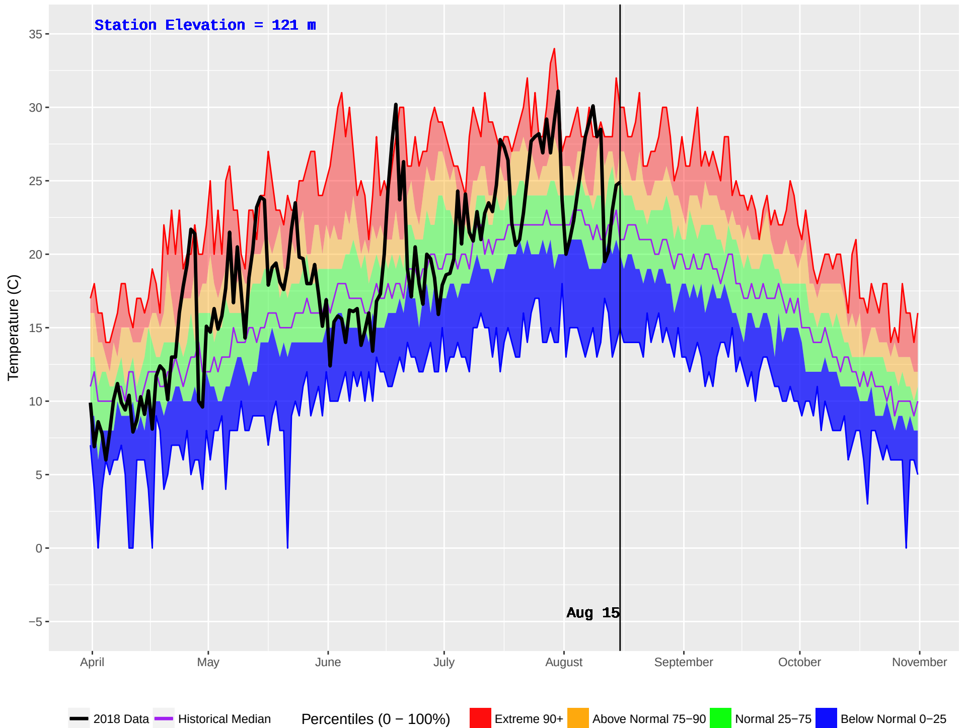
BOWSER (56) : Historical (1985–2016) and Current (2018) Daily Temperature
